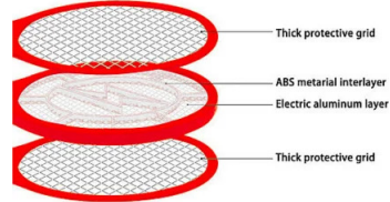
Triple-Layer Safety Mesh
